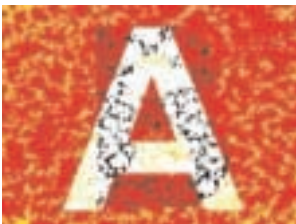
Texture - Chunks
